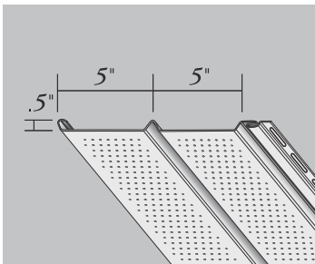
Vented panels provide air flow needed for efficient attic ventilation.
