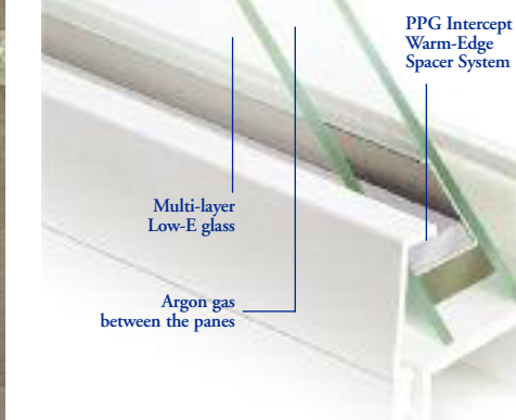
Alside new construction windows combine multi-layer Low-E glass, argon gas and PPG Intercept Warm-Edge Spacer System to provide maximum energy savings.
